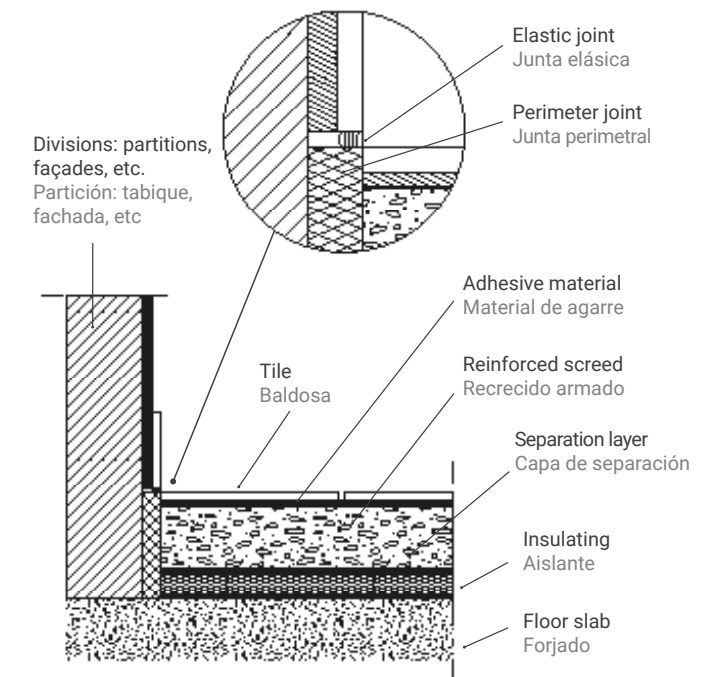
Detail of perimeter joint with sealant | Detalle de junta perimetral con sellante (UNE 138002:2017)
